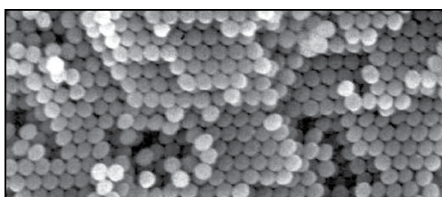
SEM photograph of ANGSTROMSPHERE™ uniform silica spheres
