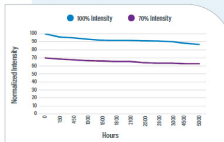
Figure 5. LED Degradation Testing - PrimeCure®
